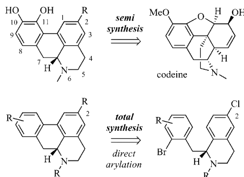
Scheme 1. Semi-synthetic and synthetic routes to C2 aporphine analogues.
