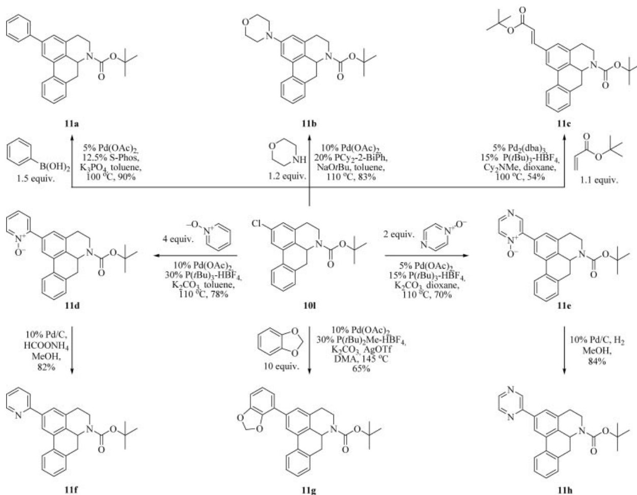
Scheme 4. Formation of C2 aporphine analogues through various cross-coupling reactions.
