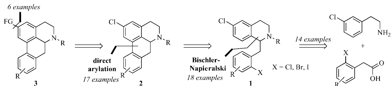
Scheme 2. Direct arylation as a convergent and divergent strategy for aporphine synthesis.
