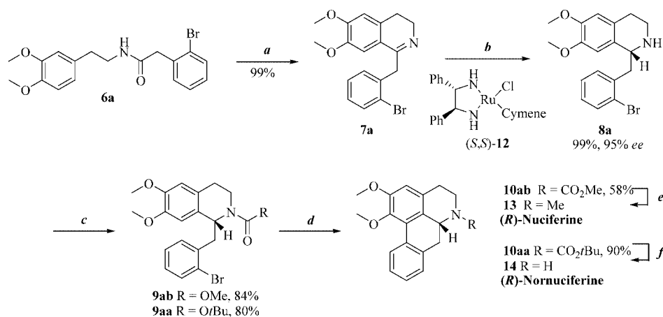
Scheme 5. a) Reaction conditions: (a) POCl 3 , DCM, reflux; b) (S,S)- 12 (5 mol-%), HCO 2 H/NEt 3 , DMF, room temp., 60 min, 99% over 2 steps, 95% ee; c) (ROC) 2 O, DMAP (cat.), i Pr 2 EtN, yield indicated; d) Pd(OAc) 2 (5 mol-%), 2-(diphenylphosphanyl)-2'-(dimethylamino)-biphenyl (10 mol-%), KOAc (2.0 equiv.), DMA, 130 °C, 4 h, yield indicated; (e) LAH, THF, 0 °C to room temp., 24 h, 88%; (f) trifluoroacetic acid (13 equiv.), DCM, room temp., 1 h, 53%.
