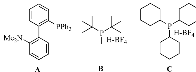
Scheme 3. Ligands employed for direct arylation.
